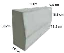
Kansteen 9.14.60 9,5/14 x 30 x 60 1,67 pcs/m 1
