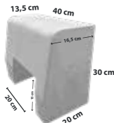
Kansteen 16.20 in 13,5/20 cm x 30 cm x 40 cm Inlet 20 cm x 15 cm (2.5 pcs/m 1 )
