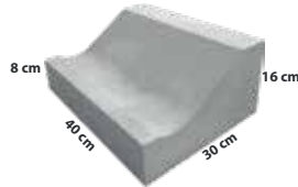
Kansteen S 8/16 x 30 cm x 40 cm 2.5 pcs/m 1
