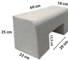
Kansteen DKI in 18/22 x 25 cm x 60 cm Inlet 12,5 cm x 29 cm 1.67 pcs/m 1
