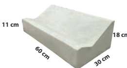
Kansteen S 11.18.60 11/18 x 30 cm x 60 cm 1,67 pcs/m 2
