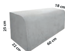
Kansteen DKI 18/22 x 25 cm x 60 cm 1.67 pcs/m 2
