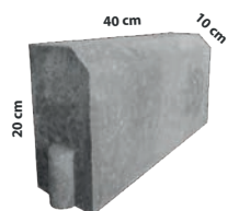
Kansteen Jepit 10 cm x 20 cm x 40 cm 2.5 pcs/m 2
