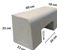
Kansteen DKI in 18/22 x 25 cm x 60 cm Inlet 12,5 cm x 29 cm 1.67 pcs/m 2
