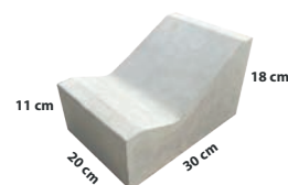
Kansteen S 11.18.20 11/18 x 30 cm x 20 cm 5 pcs/m 2
