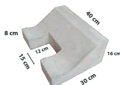
Kansteen S in 8/16 x 30 cm x 40 cm Inlet 15 cm x 12 cm 2.5 pcs/m 2
