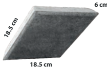
Wajik (3D) 18,5 cm x 18,5 cm Tebal 6 cm 34 pcs/m2
