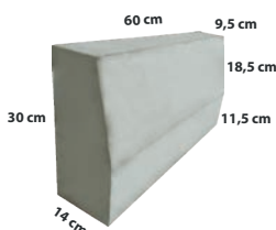
Kansteen 9.14.60 9,5/14 x 30 x 60 1,67 pcs/m 2
