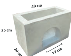
Grill Box 40 cm x 20 cm x 25 cm Inlet 17 cm
