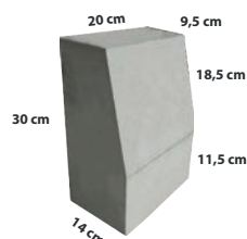
Kansteen 9.14.20 9,5/14 x 30 cm x 20 cm 5 pcs/m 2
