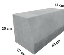
Kansteen 13.17 13/17 cm x 20 cm x 40 cm (2.5 pcs/m 2 )
