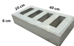
Grill 20 cm x 40 cm x 8 cm Inlet 4 cm x 11 cm
