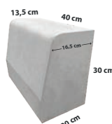
Kansteen 16.20 13,5/20 cm x 30 cm x 40 cm (2.5 pcs/m 2 )
